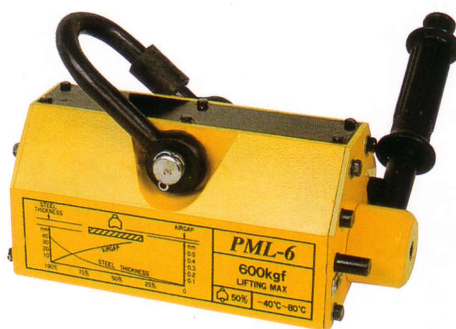
Magnetic Lifter
